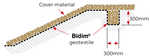
Figure 2. Slopes
