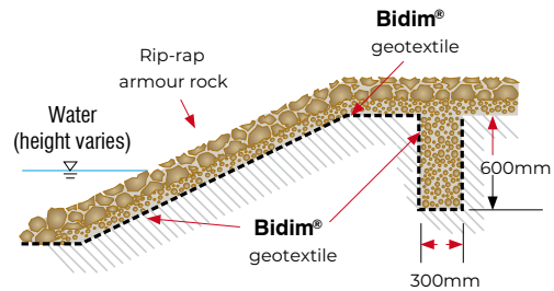
Figure 3. Revetments
